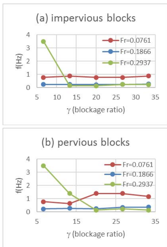
Figure 10. Relationship between blockage ratio and maximum transient velocity frequency
