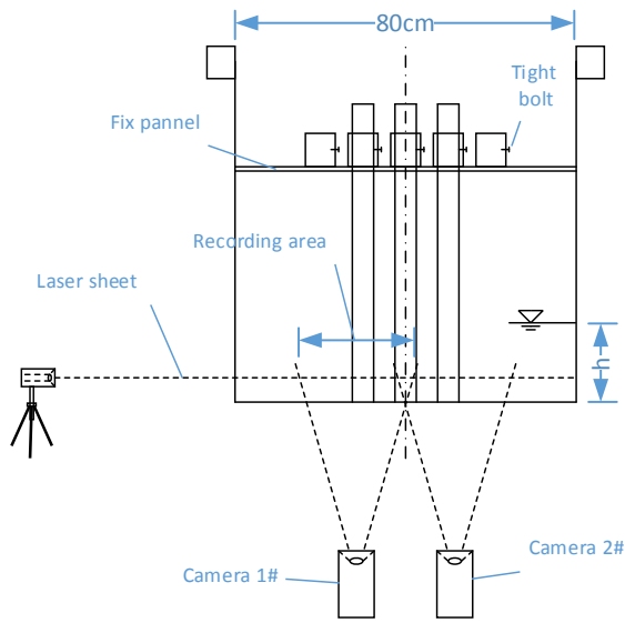
Figure 3. Testing area profile
