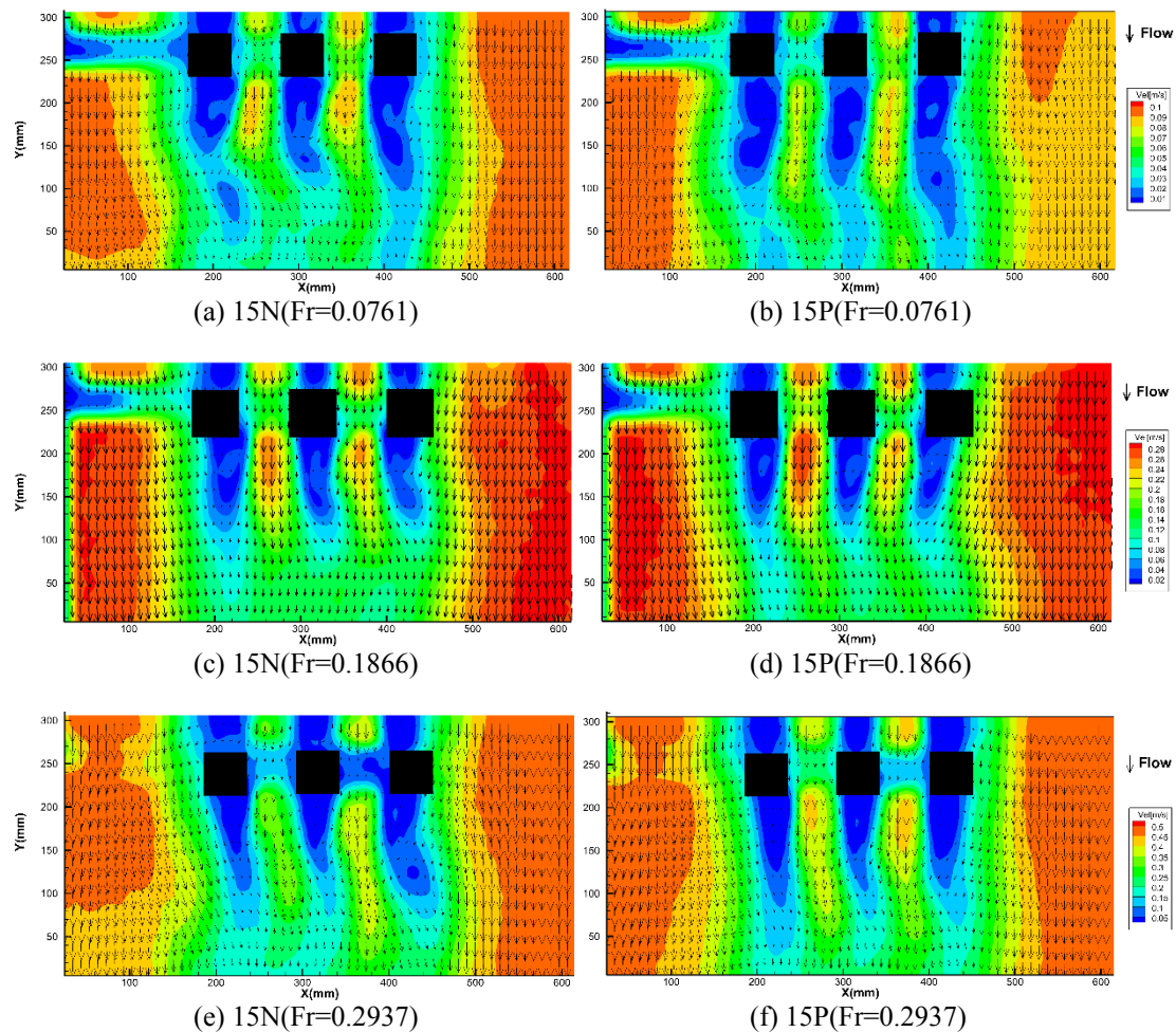
Figure 9. Flow pattern behind the blocks ( \gamma = 33.33\% )
