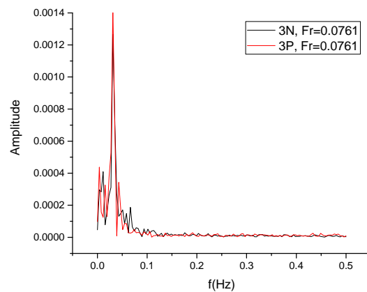
Fig. 8. Frequency of transient velocity for Fr=0.0761
