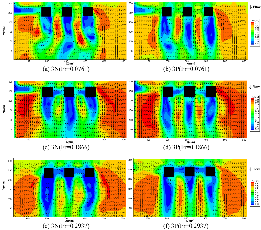
Figure 7. Flow pattern behind the blocks( \gamma=6.67\% )
