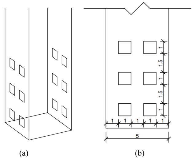
Figure 4. Pervious building (a) 3D view; (b) square pervious holes dimensions
