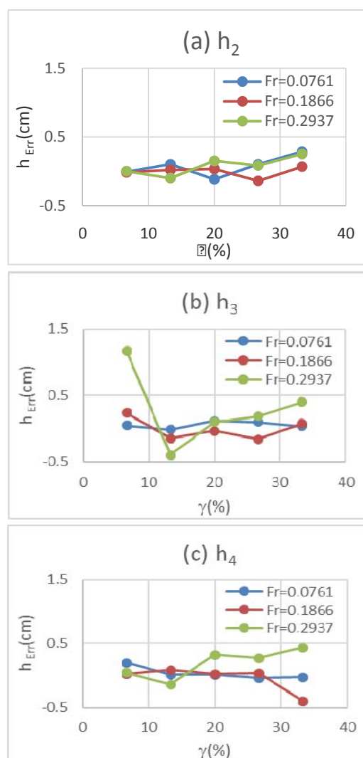
Figure 6. Relationship between blockage ratio ( \gamma ) and depths difference( h_{err} ) ( h_2, h_3, h_4 denote the left, centre, right column blocks, respectively)
