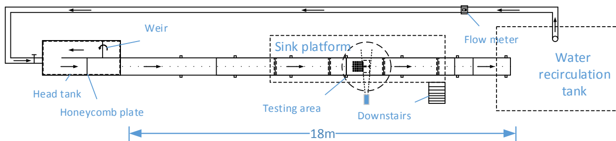
Figure 1. Experimental facilities and setup
