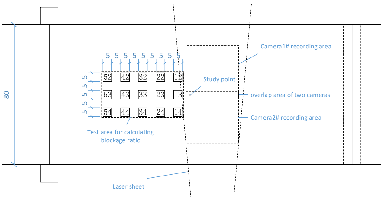
Figure 2. Details of testing area and building blocks indexing (Dimension in cm)
